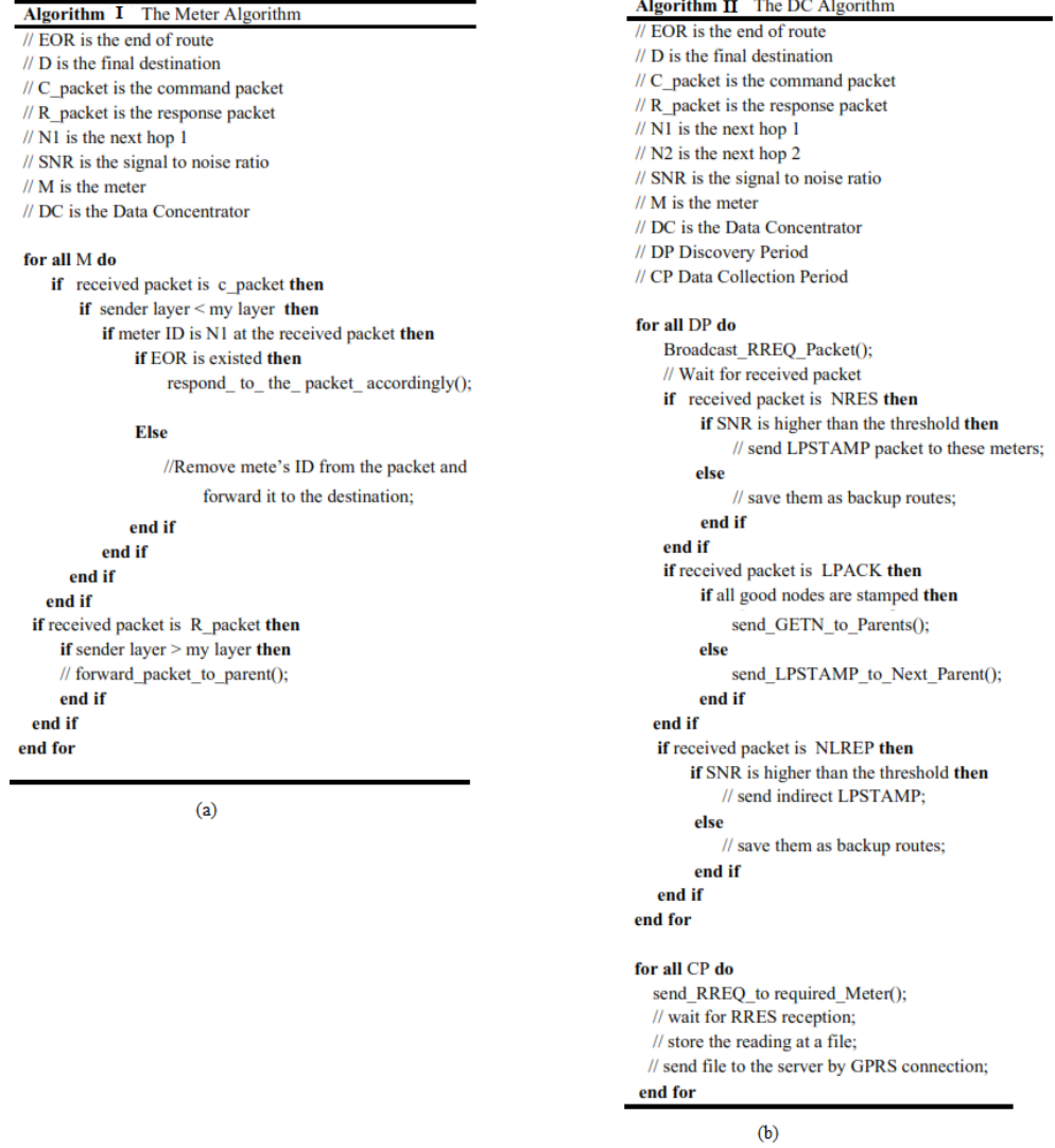
Fig. 3. (a) Meter algorithm. (b) DC algorithm
