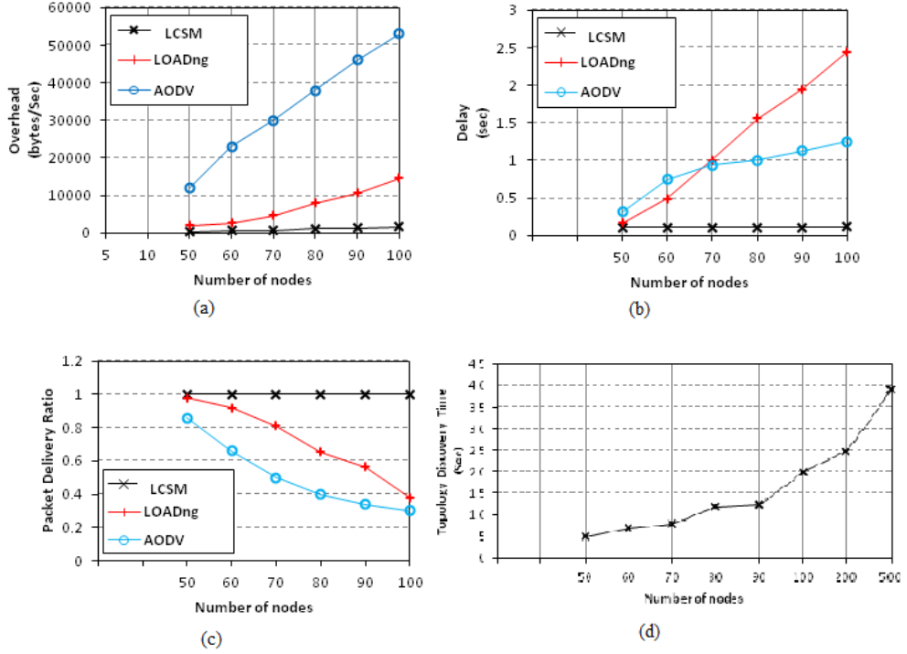
Fig. 4. (a) Routing overhead. (b) End-to-End delay. (c) Packet delivery ratio. (d) Topology discovery time at 2400 bps.
